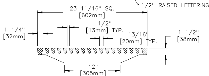
GRATE SECTION
