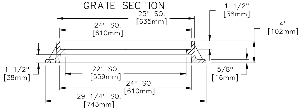
FRAME SECTION
