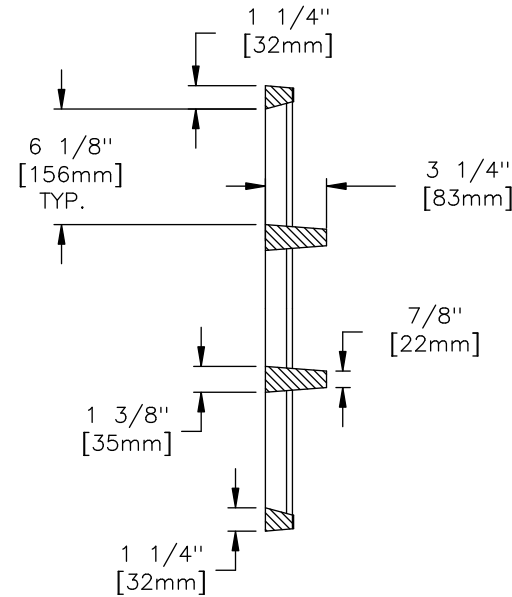
GRATE SECTION
